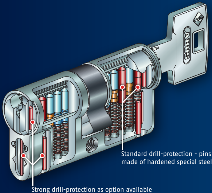
Cylinder illustration with optional drill-protection
